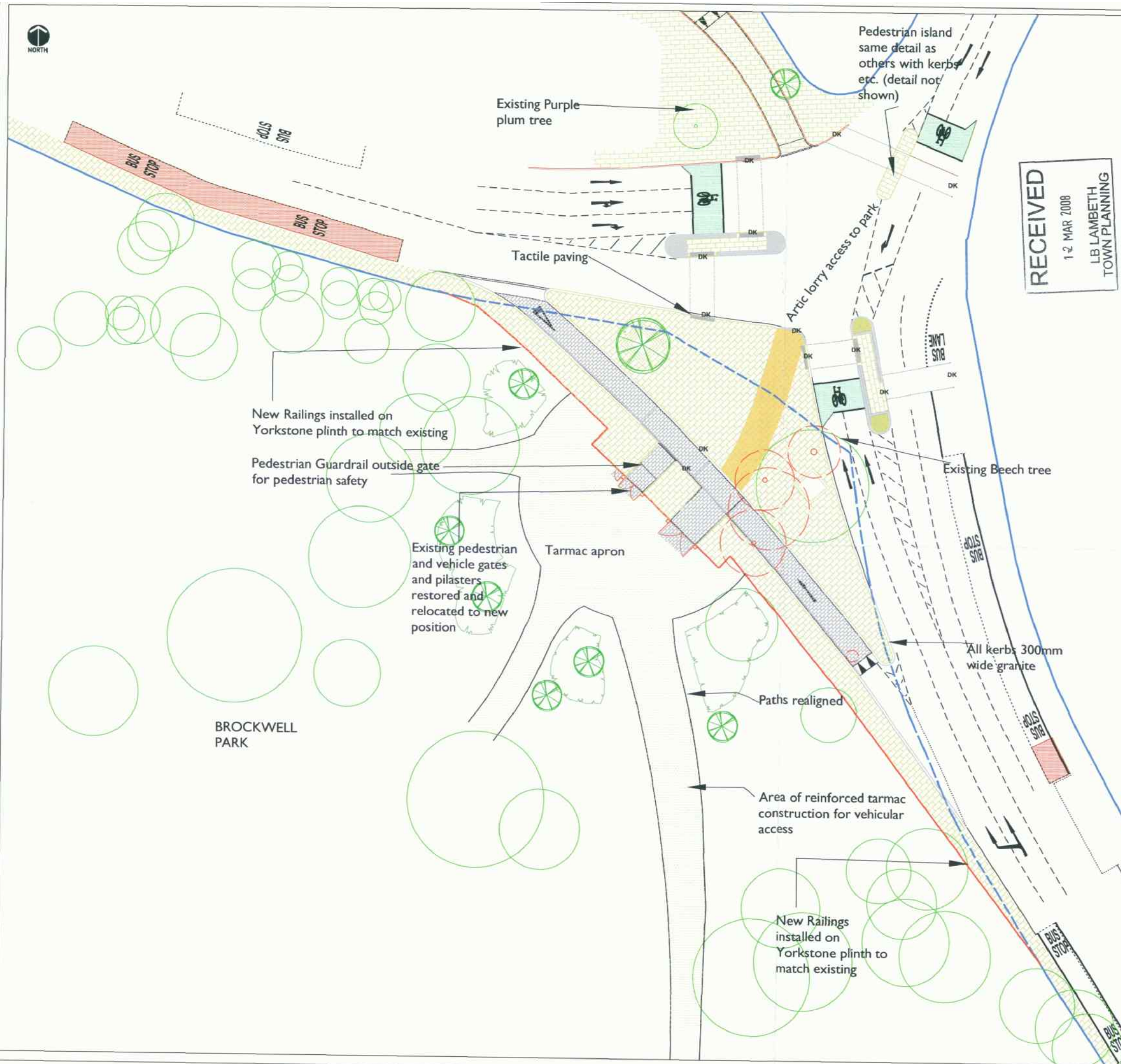
Typical pedestrian crossing point
